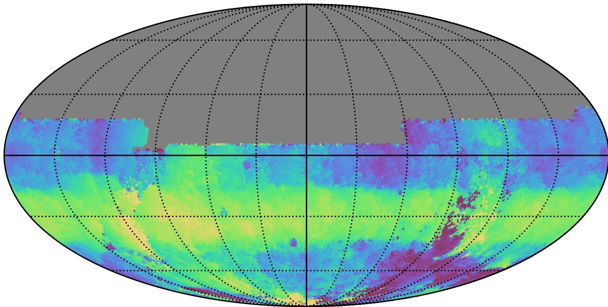
ddf_loaded_half_fl8_v3.4_10yrs All sky u band: Median HA
