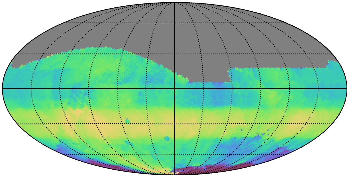
ddf_loaded_half_fl8_v3.4_10yrs All sky r band: Median HA
