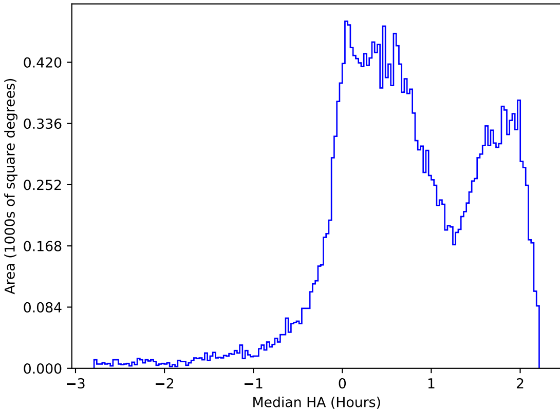
ddf_loaded_half_fl8_v3.4_10yrs All sky r band: Median HA
