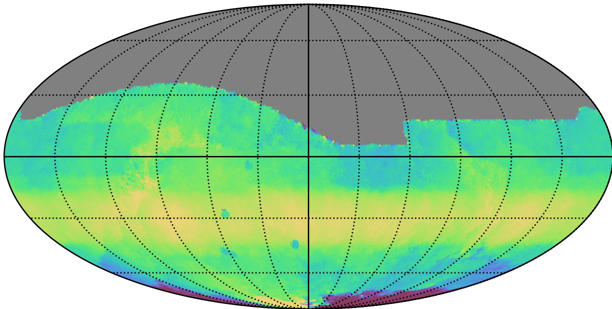
ddf_loaded_half_fl8_v3.4_10yrs All sky i band: Median HA
