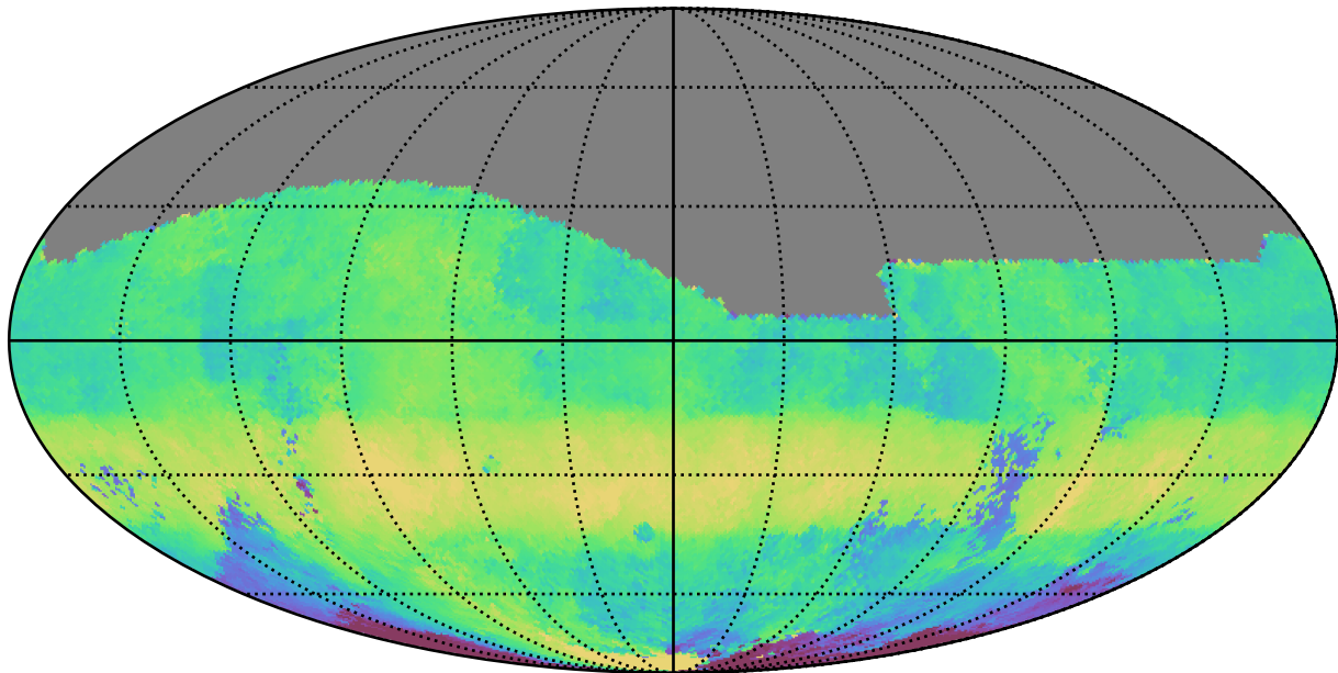
ddf_loaded_half_f18_v3.4_10yrs All sky g band: Median HA
