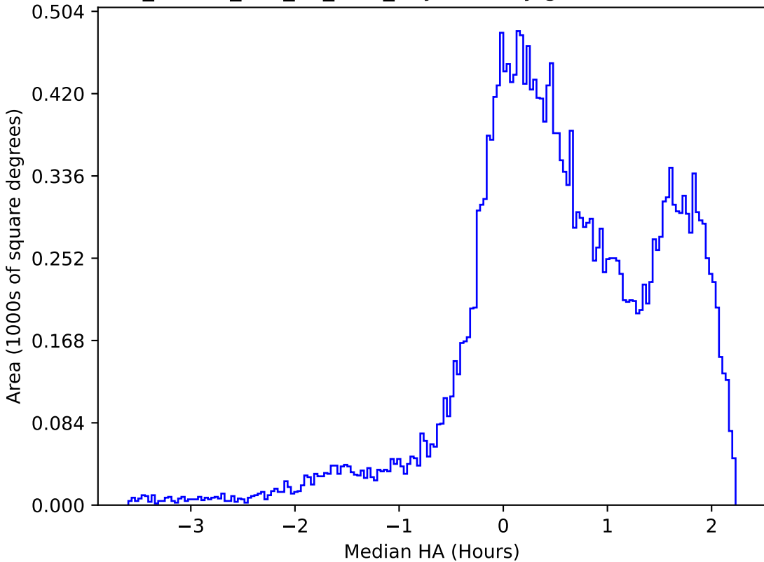
ddf_loaded_half_fl8_v3.4_10yrs All sky g band: Median HA
