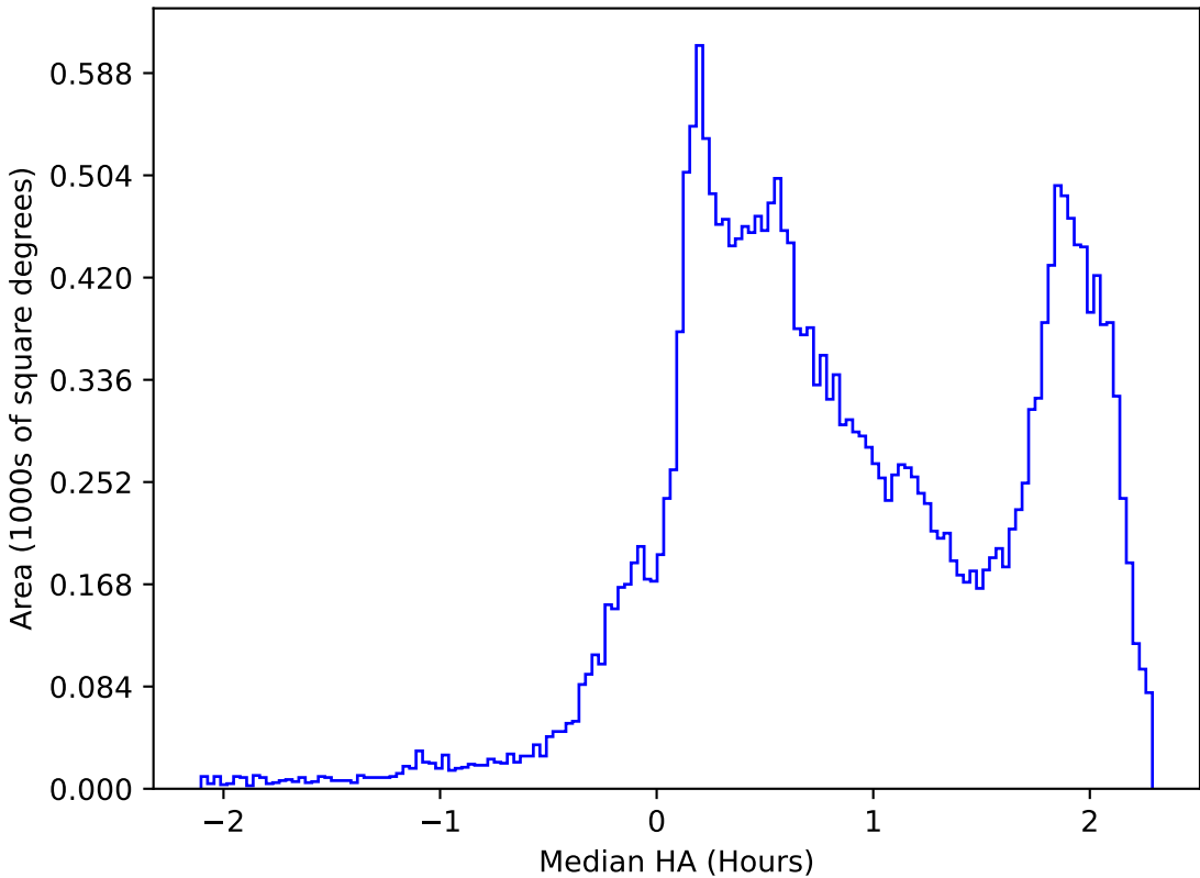
ddf_loaded_half_fl8_v3.4_10yrs All sky all bands: Median HA
