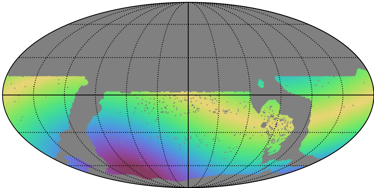
ddf_loaded_half_fl8_v3.4_10yrs WFD y band: Max solarElong
