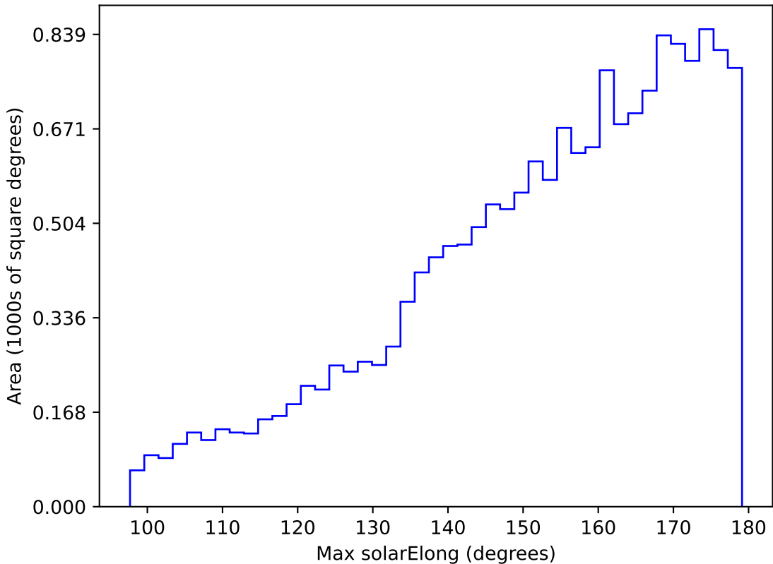
ddf_loaded_half_fl8_v3.4_10yrs WFD u band: Max solarElong
