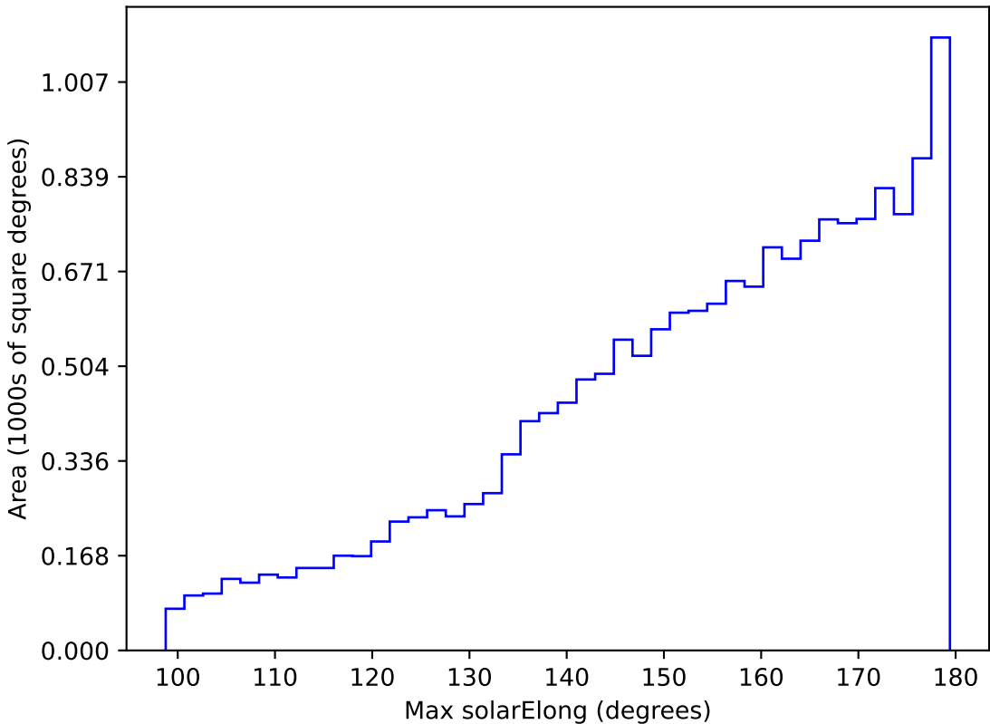
ddf_loaded_half_fl8_v3.4_10yrs WFD r band: Max solarElong
