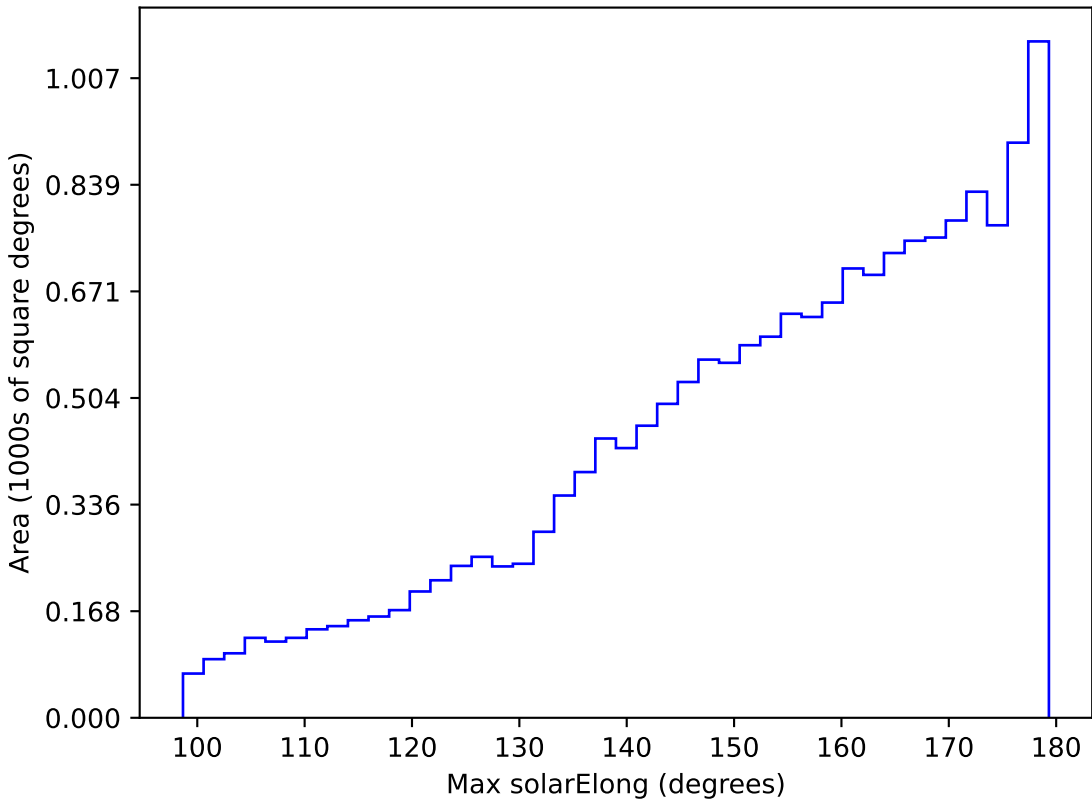
ddf_loaded_half_fl8_v3.4_10yrs WFD i band: Max solarElong
