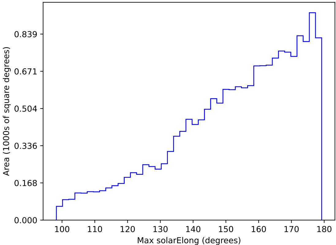
ddf_loaded_half_fl8_v3.4_10yrs WFD g band: Max solarElong
