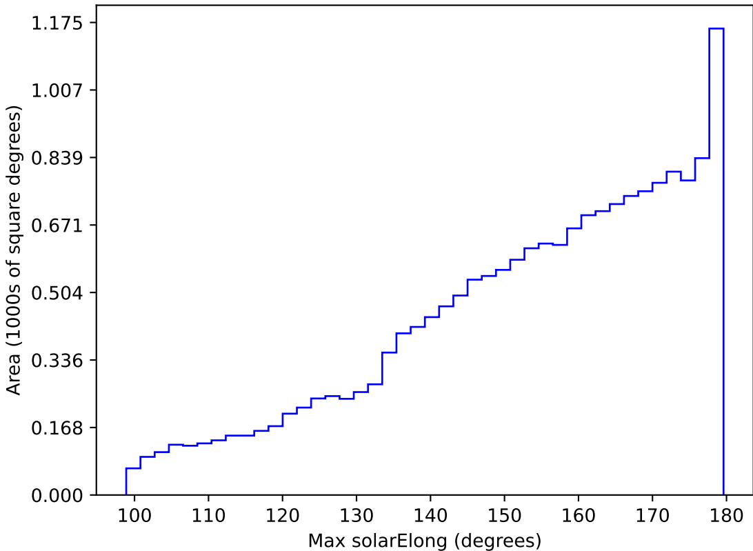
ddf_loaded_half_fl8_v3.4_10yrs WFD all bands: Max solarElong
