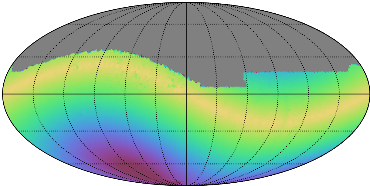
ddf_loaded_half_fl8_v3.4_10yrs All sky z band: Max solarElong
