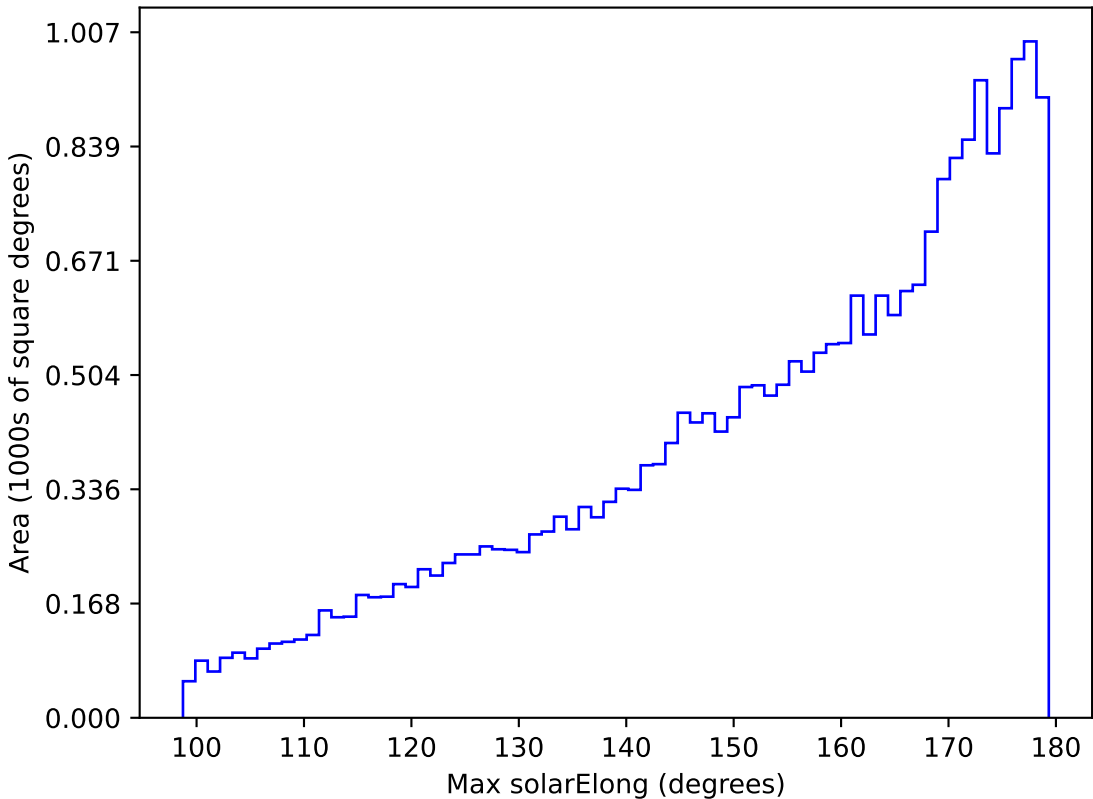
ddf_loaded_half_fl8_v3.4_10yrs All sky z band: Max solarElong
