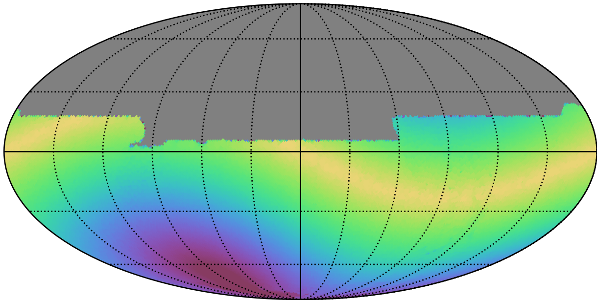
ddf_loaded_half_fl8_v3.4_10yrs All sky y band: Max solarElong
