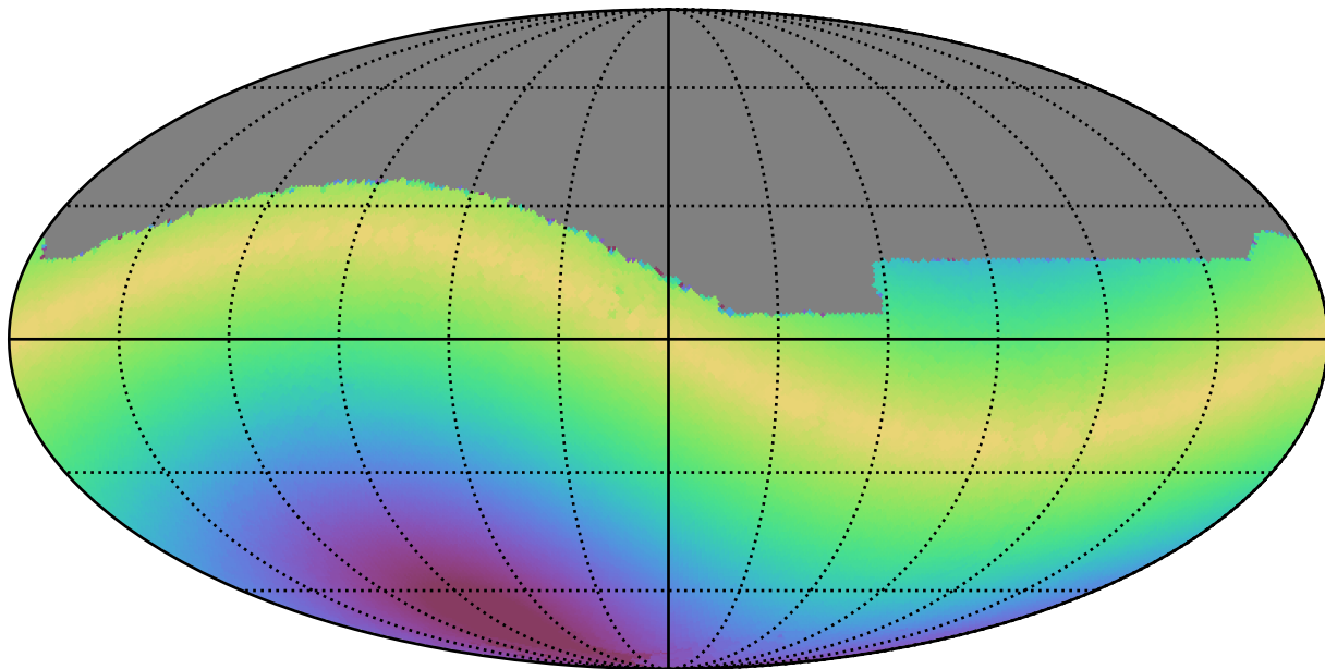
ddf_loaded_half_fl8_v3.4_10yrs All sky i band: Max solarElong
