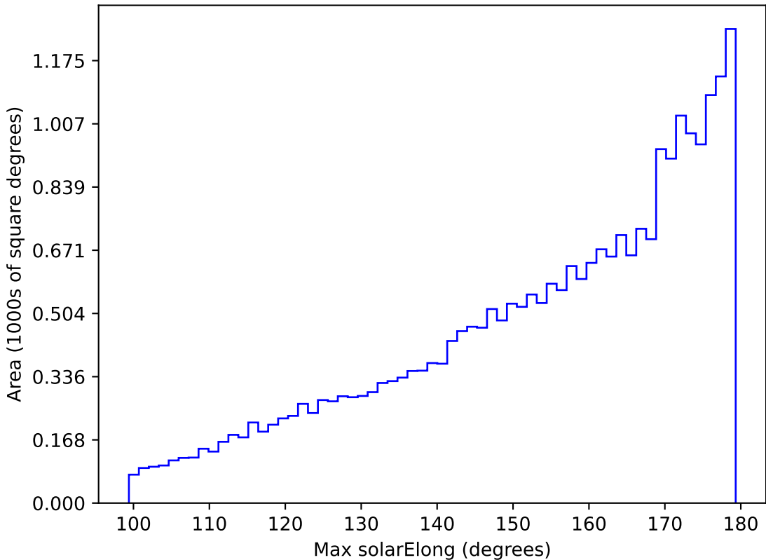
ddf_loaded_half_fl8_v3.4_10yrs All sky i band: Max solarElong
