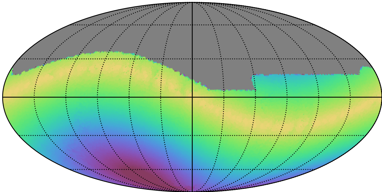
ddf_loaded_half_fl8_v3.4_10yrs All sky g band: Max solarElong
