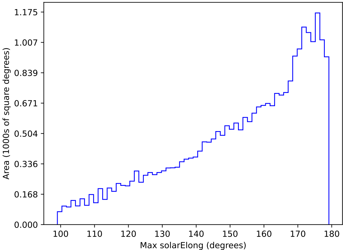
ddf_loaded_half_fl8_v3.4_10yrs All sky g band: Max solarElong
