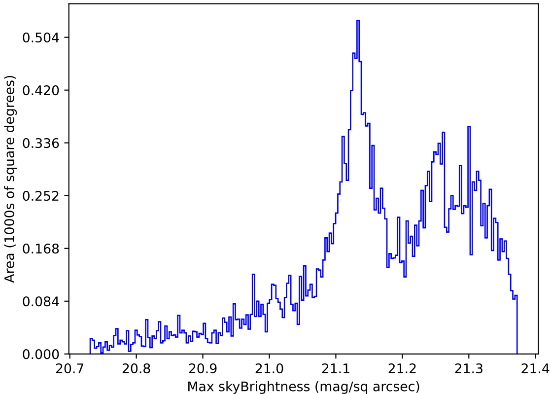
ddf_loaded_half_fl8_v3.4_10yrs Yr 1 r band: Max skyBrightness
