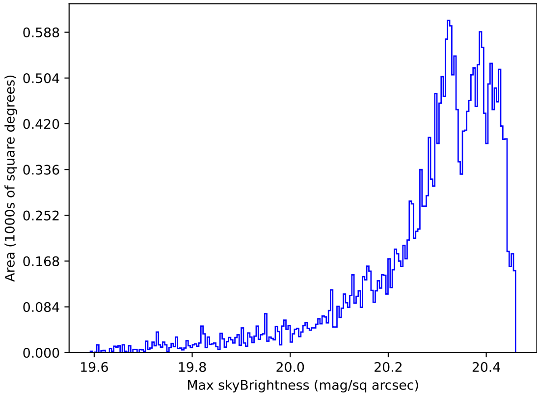
ddf_loaded_half_fl8_v3.4_10yrs Yr 1 i band: Max skyBrightness
