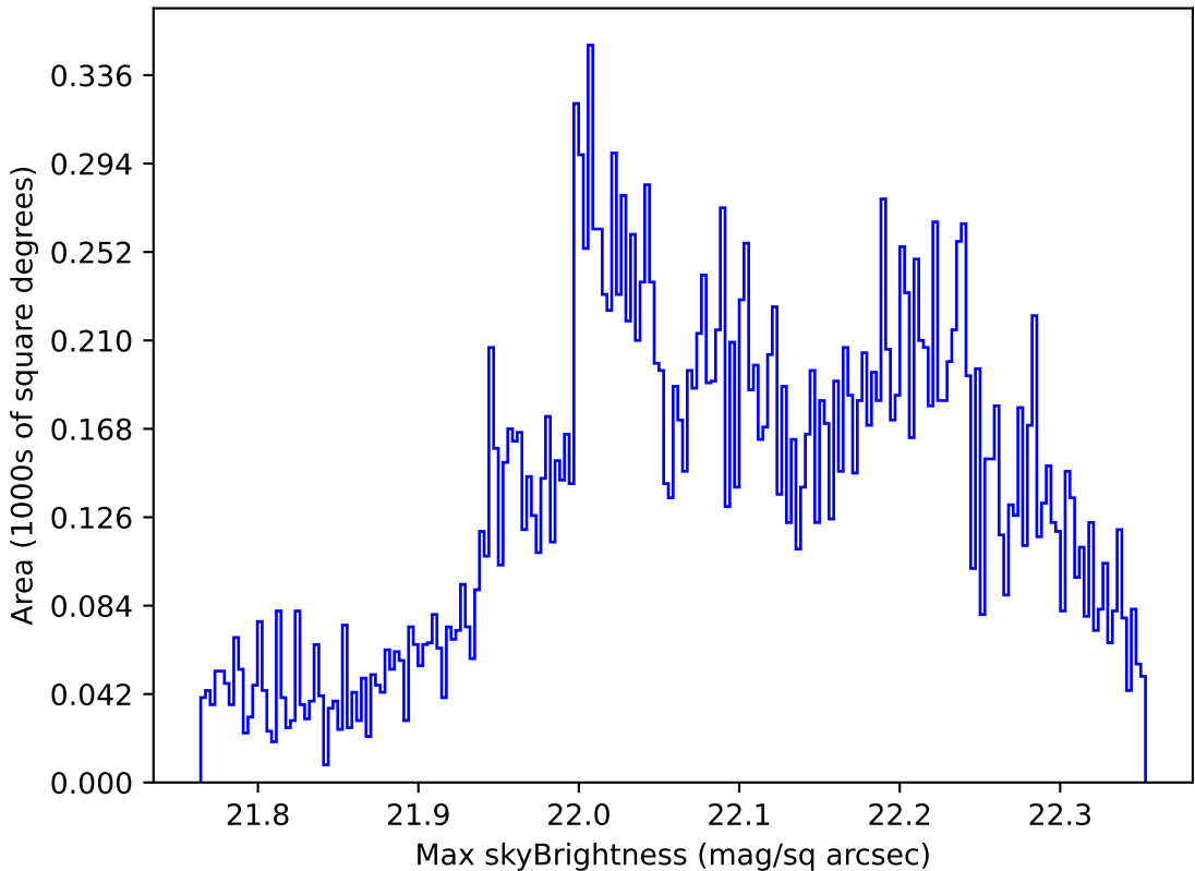
ddf_loaded_half_fl8_v3.4_10yrs Yr 1 g band: Max skyBrightness
