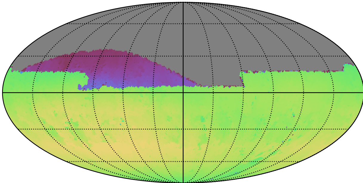
ddf_loaded_half_fl8_v3.4_10yrs Yr 1 all bands: Max skyBrightness
