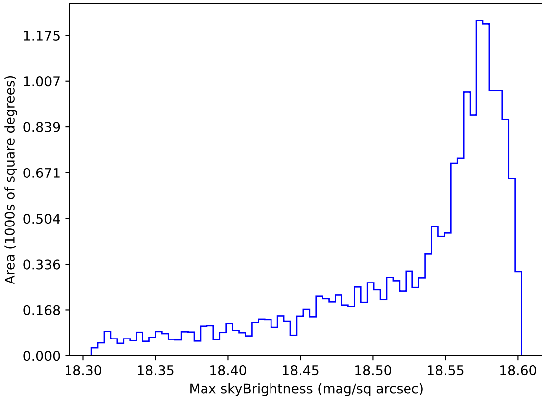
ddf_loaded_half_fl8_v3.4_10yrs WFD y band: Max skyBrightness
