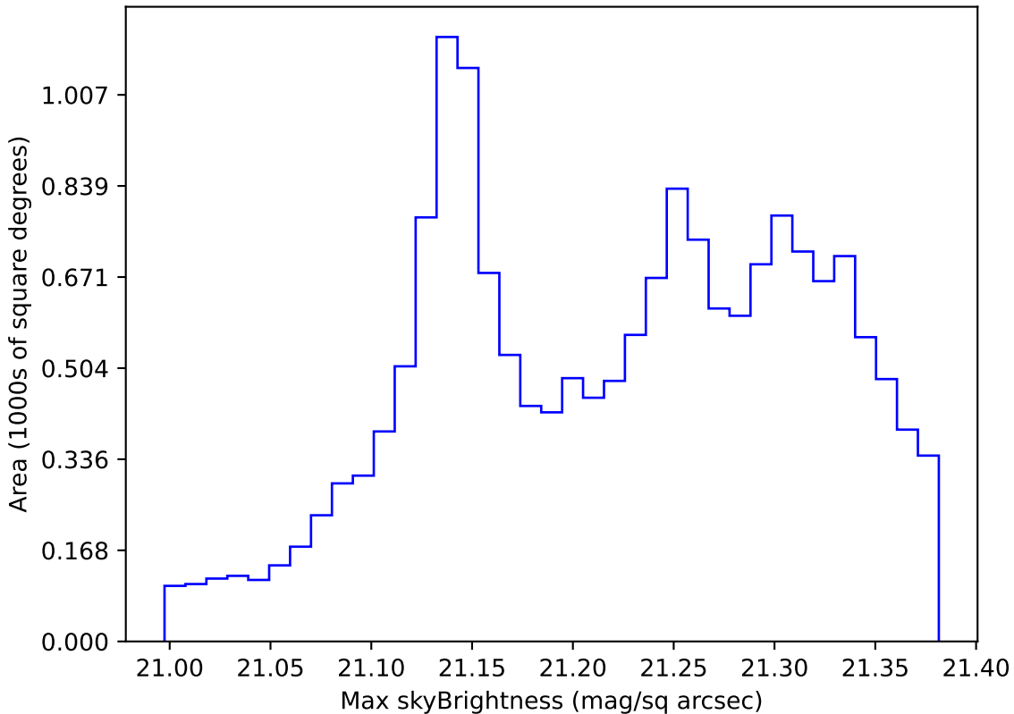
ddf_loaded_half_fl8_v3.4_10yrs WFD r band: Max skyBrightness
