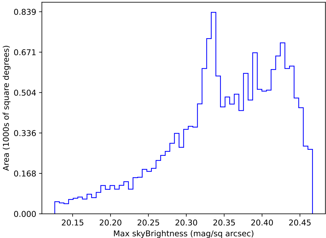
ddf_loaded_half_fl8_v3.4_10yrs WFD i band: Max skyBrightness
