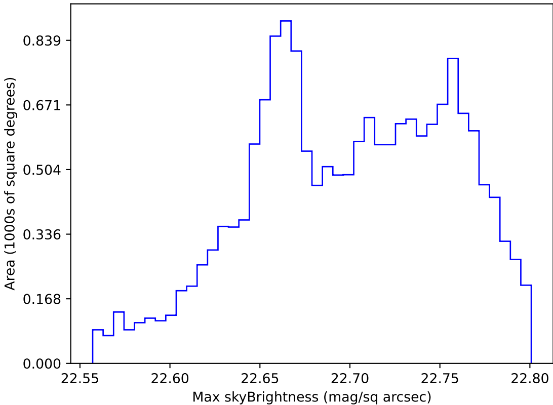
ddf_loaded_half_fl8_v3.4_10yrs WFD all bands: Max skyBrightness
