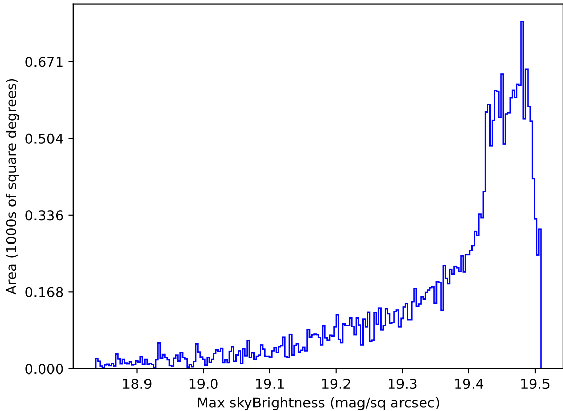
ddf_loaded_half_fl8_v3.4_10yrs All sky z band: Max skyBrightness
