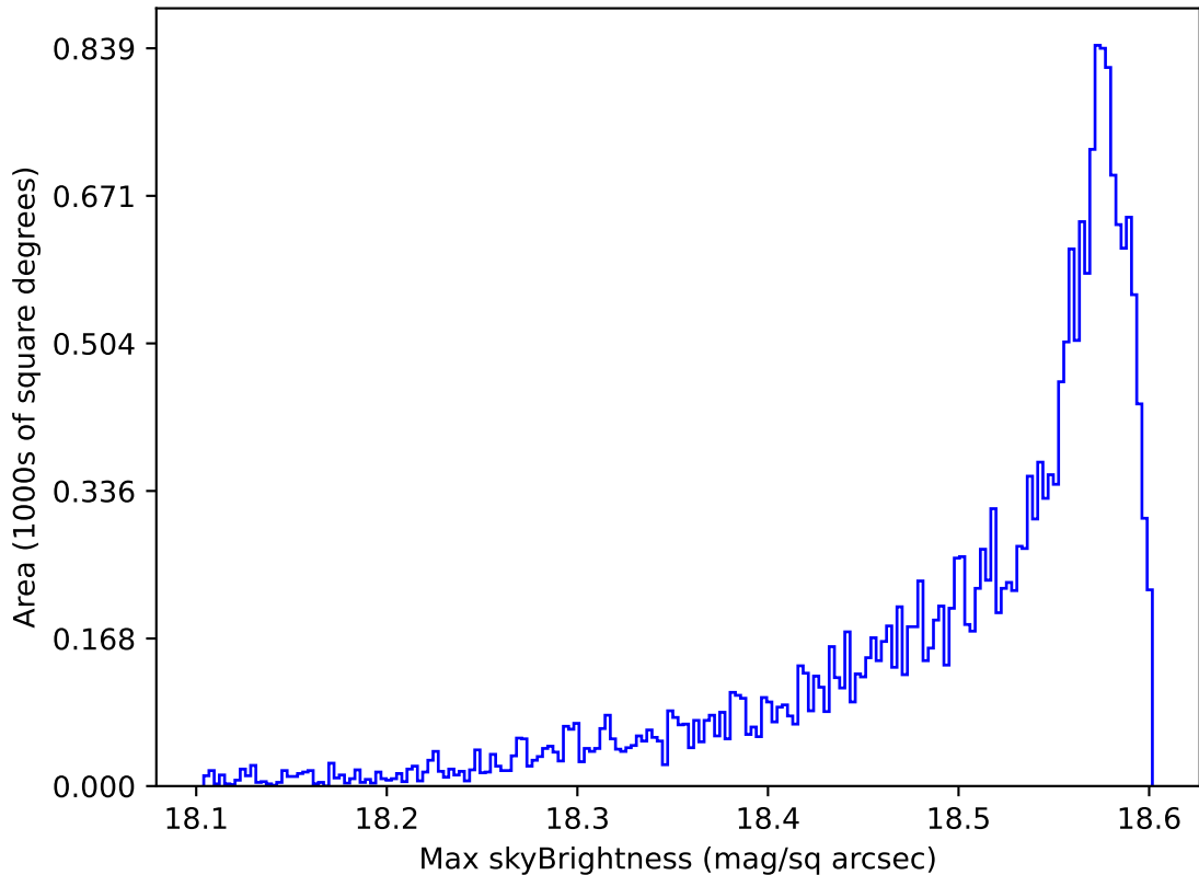
ddf_loaded_half_fl8_v3.4_10yrs All sky y band: Max skyBrightness
