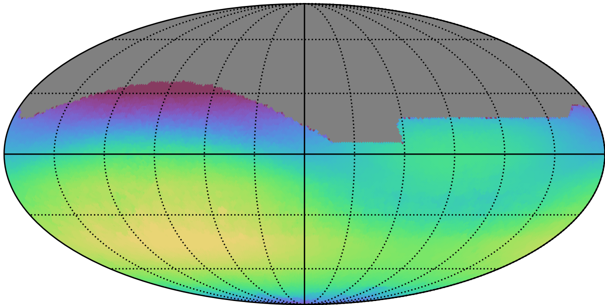
ddf_loaded_half_fl8_v3.4_10yrs All sky r band: Max skyBrightness
