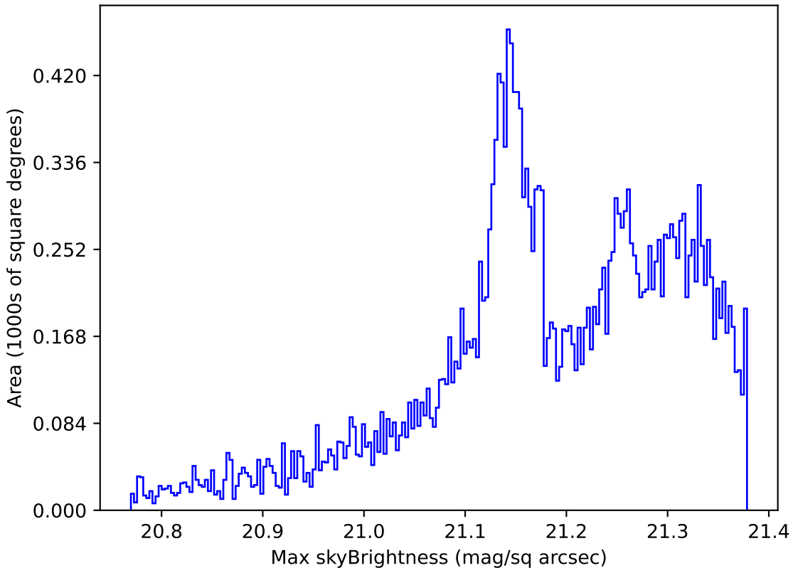
ddf_loaded_half_fl8_v3.4_10yrs All sky r band: Max skyBrightness
