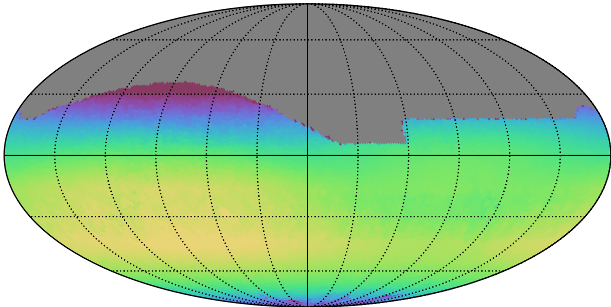
ddf_loaded_half_fl8_v3.4_10yrs All sky i band: Max skyBrightness
