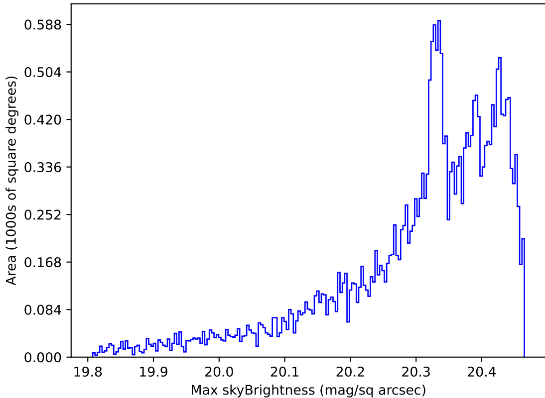
ddf_loaded_half_fl8_v3.4_10yrs All sky i band: Max skyBrightness
