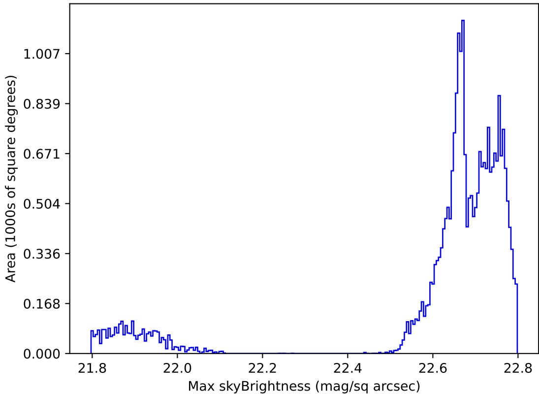
ddf_loaded_half_fl8_v3.4_10yrs All sky all bands: Max skyBrightness
