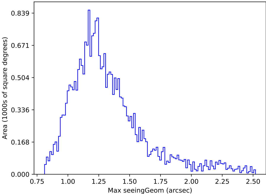
ddf_loaded_half_fl8_v3.4_10yrs Yr 1 z band: Max seeingGeom
