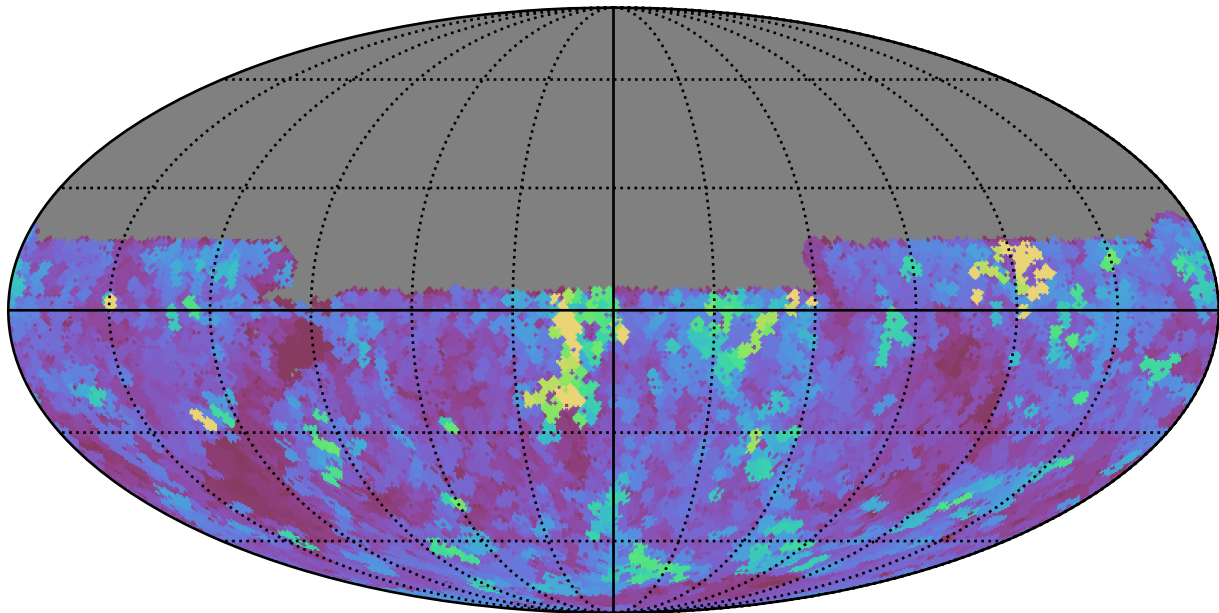
ddf_loaded_half_fl8_v3.4_10yrs Yr 1 y band: Max seeingGeom
