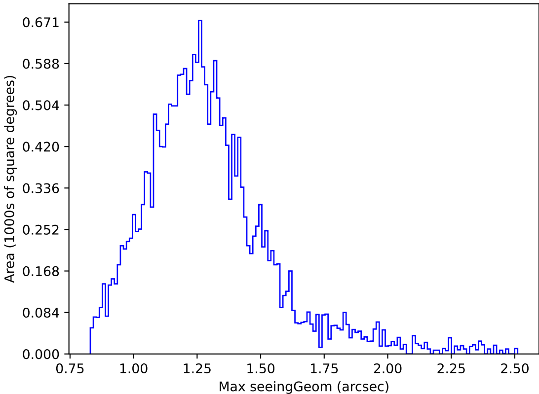
ddf_loaded_half_fl8_v3.4_10yrs Yr 1 y band: Max seeingGeom
