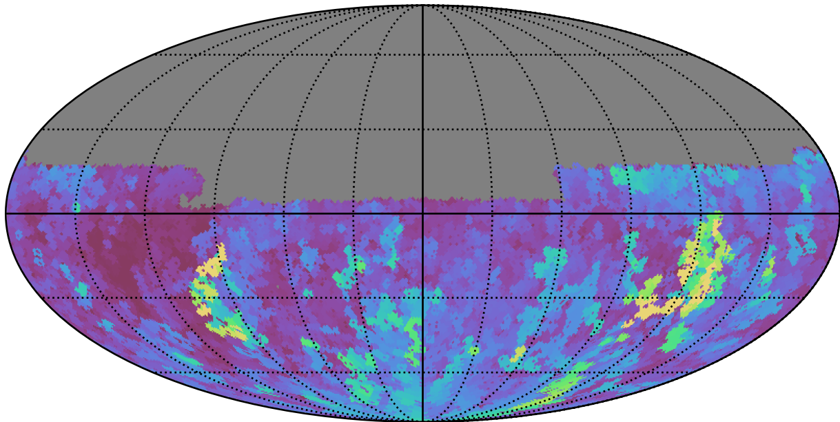
ddf_loaded_half_fl8_v3.4_10yrs Yr 1 u band: Max seeingGeom
