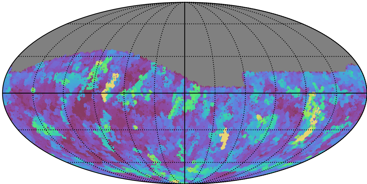
ddf_loaded_half_fl8_v3.4_10yrs Yr 1 r band: Max seeingGeom
