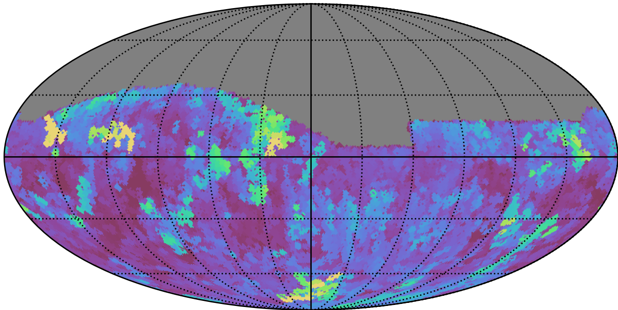
ddf_loaded_half_f18_v3.4_10yrs Yr 1 i band: Max seeingGeom
