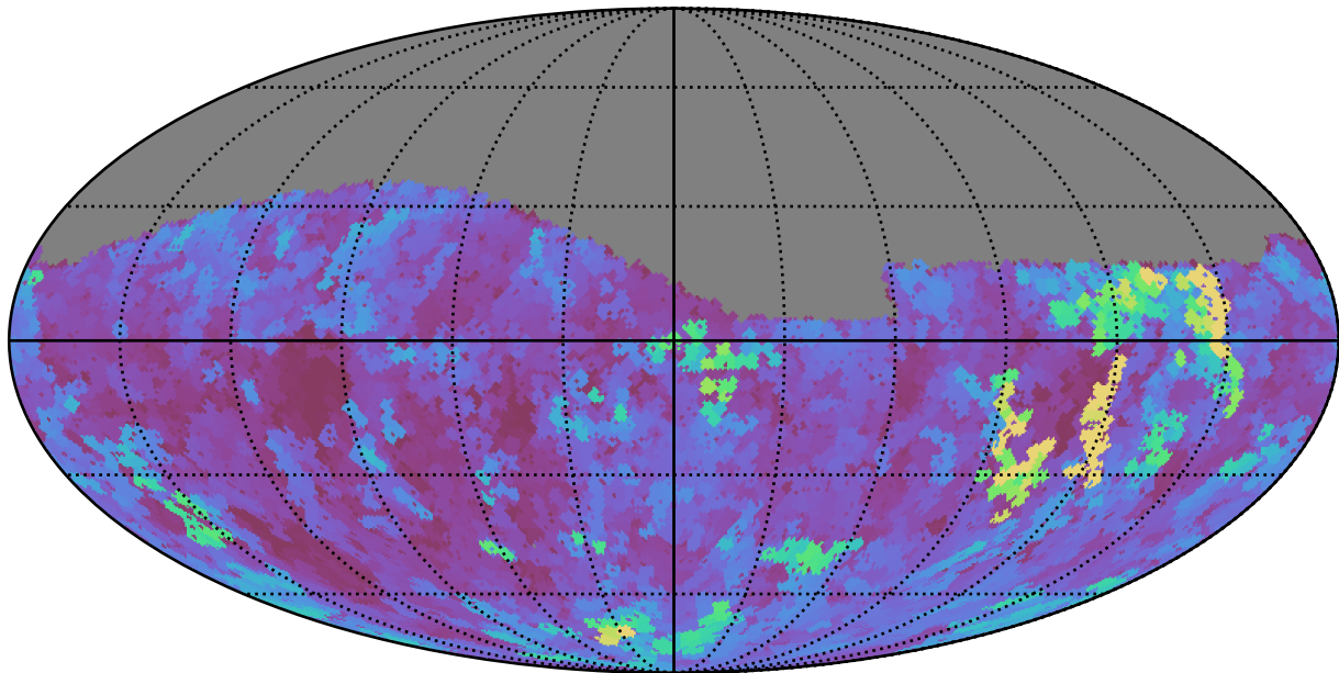
ddf_loaded_half_fl8_v3.4_10yrs Yr 1 g band: Max seeingGeom
