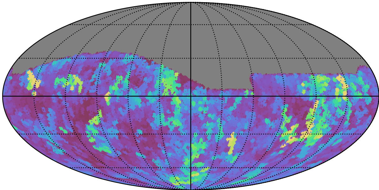
ddf_loaded_half_fl8_v3.4_10yrs Yr 1 all bands: Max seeingGeom
