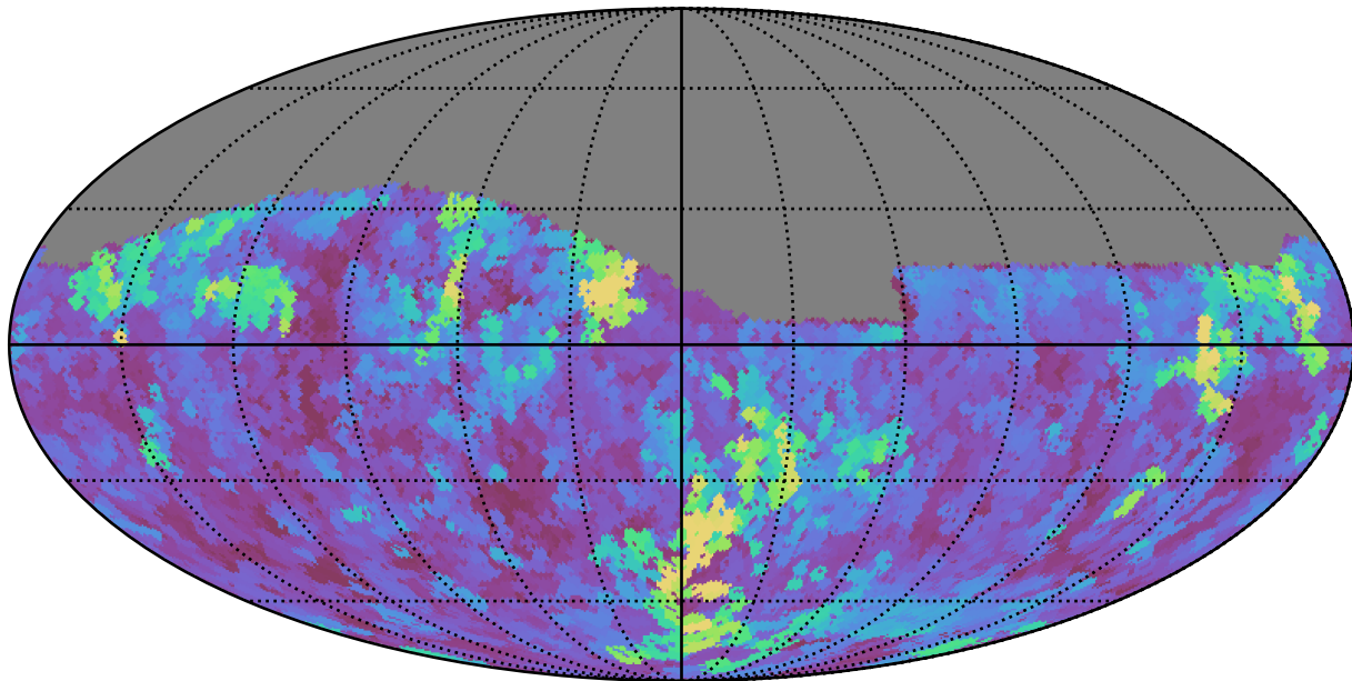
ddf_loaded_half_fl8_v3.4_10yrs Yr 1 z band: Max seeingEff
