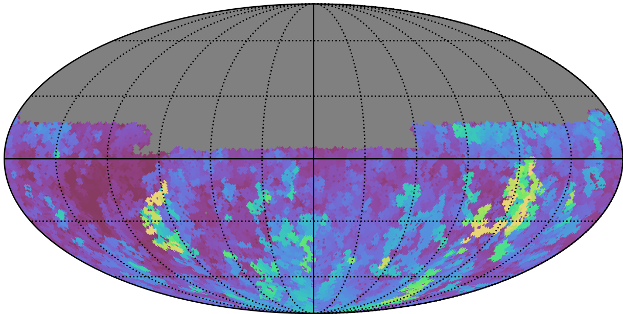
ddf_loaded_half_fl8_v3.4_10yrs Yr 1 u band: Max seeingEff
