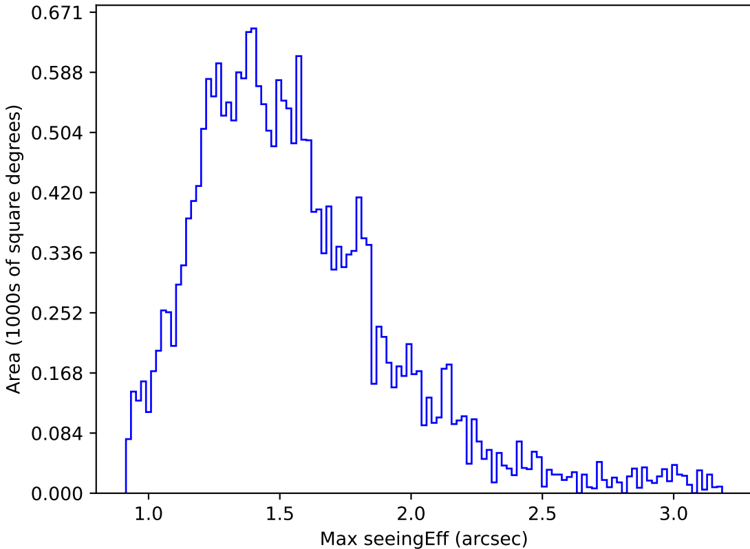
ddf_loaded_half_fl8_v3.4_10yrs Yr 1 u band: Max seeingEff
