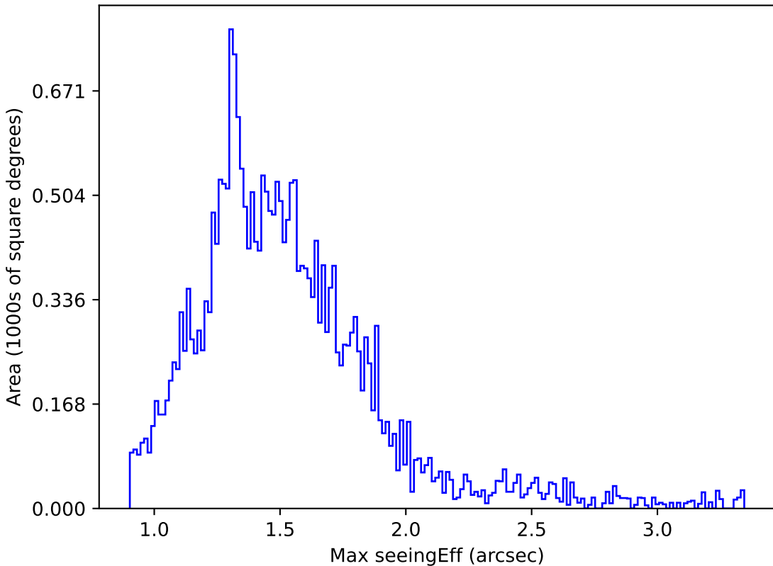
ddf_loaded_half_fl8_v3.4_10yrs Yr 1 g band: Max seeingEff
