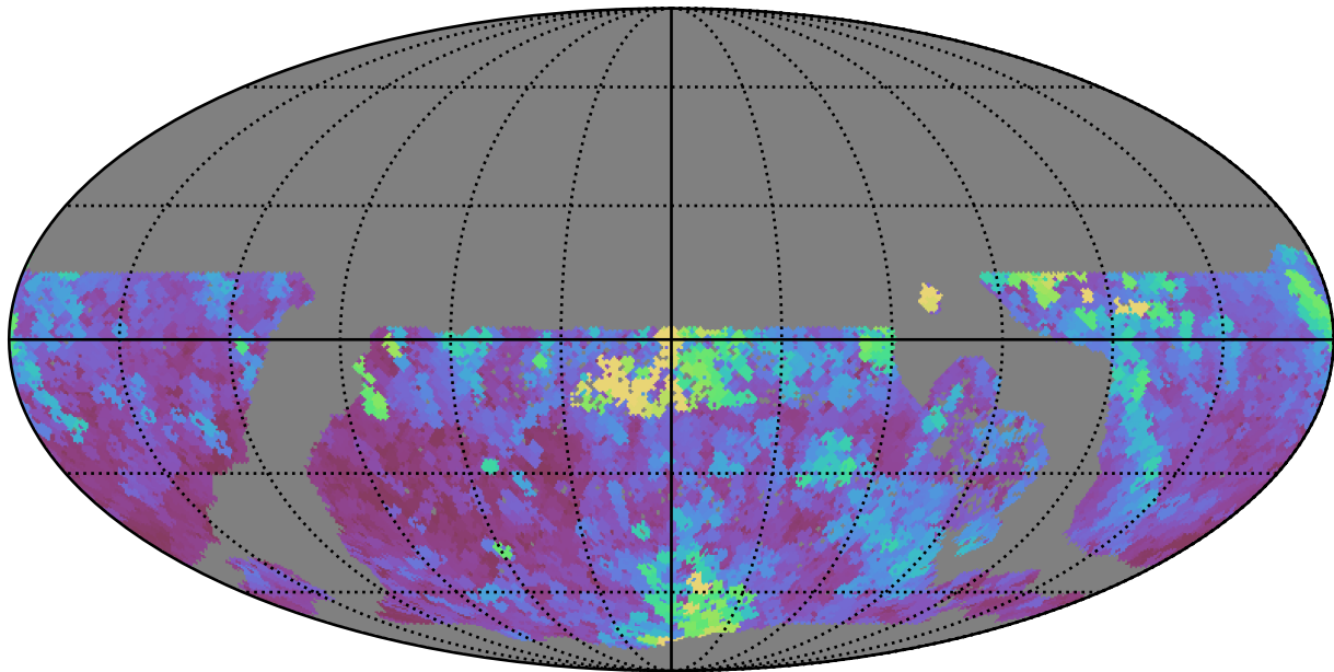
ddf_loaded_half_fl8_v3.4_10yrs WFD z band: Max seeingEff
