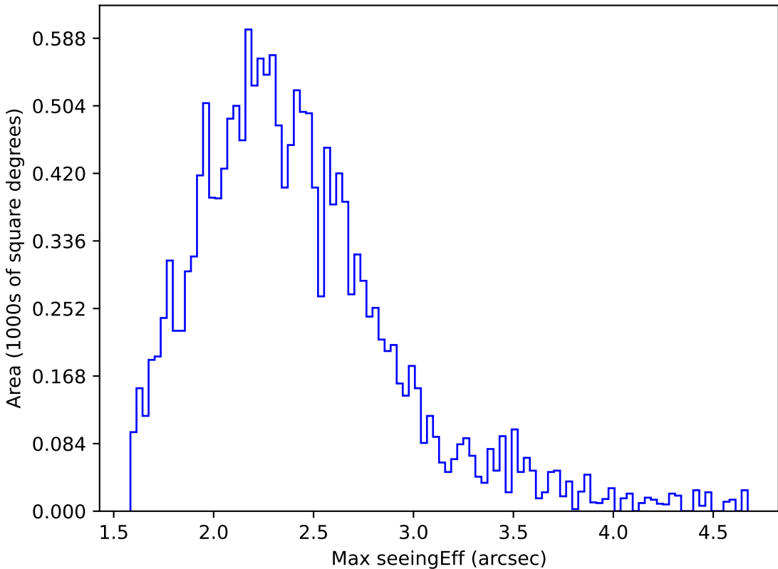
ddf_loaded_half_fl8_v3.4_10yrs WFD y band: Max seeingEff
