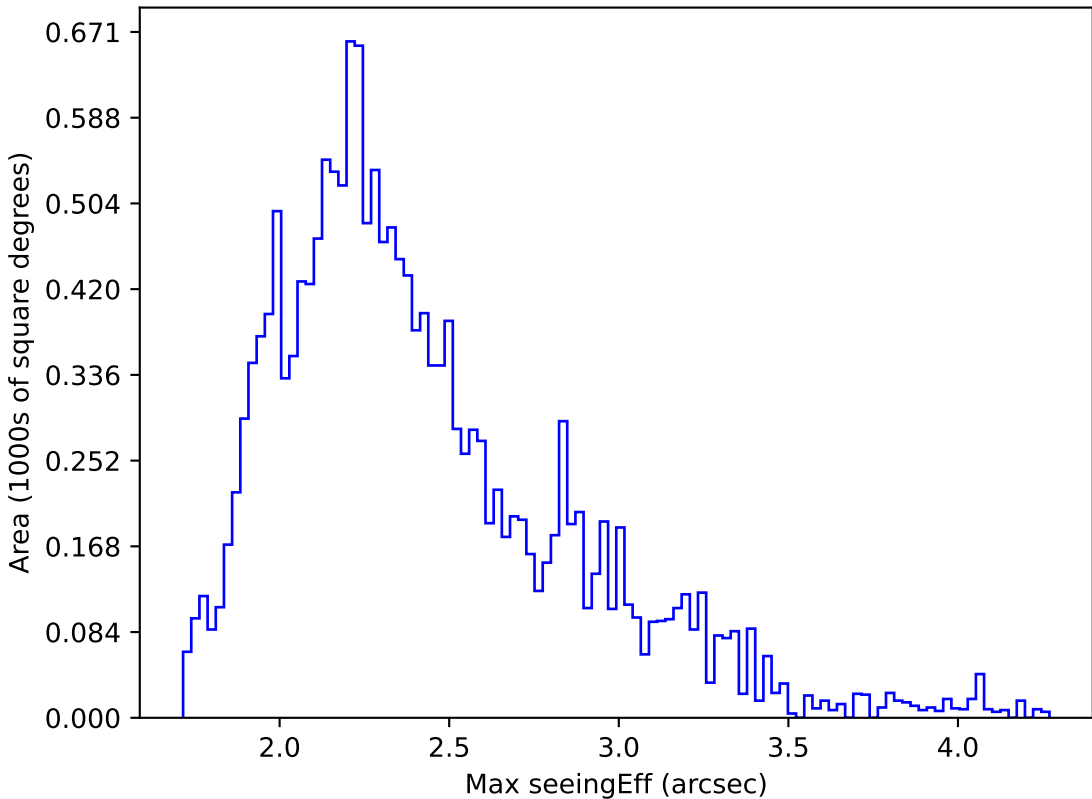
ddf_loaded_half_fl8_v3.4_10yrs WFD u band: Max seeingEff
